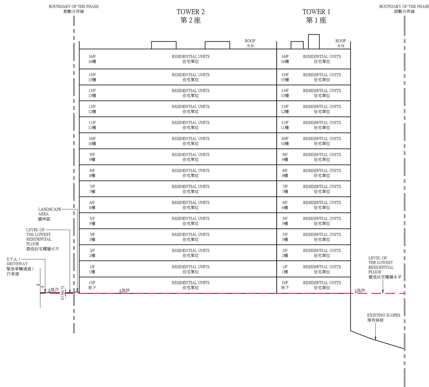
CROSS-SECTION PLAN A-A 橫截面圖A-A
