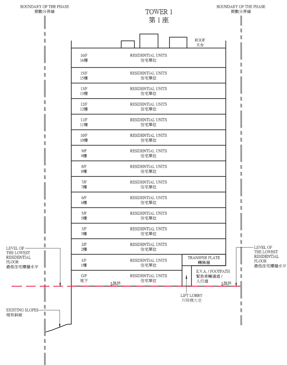
CROSS-SECTION PLAN B-B 橫截面圖B-B
