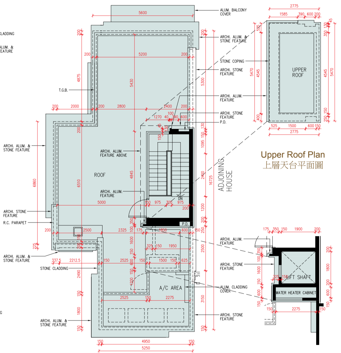
Roof Part Plan at Low Level 天台低位部分平面圖
