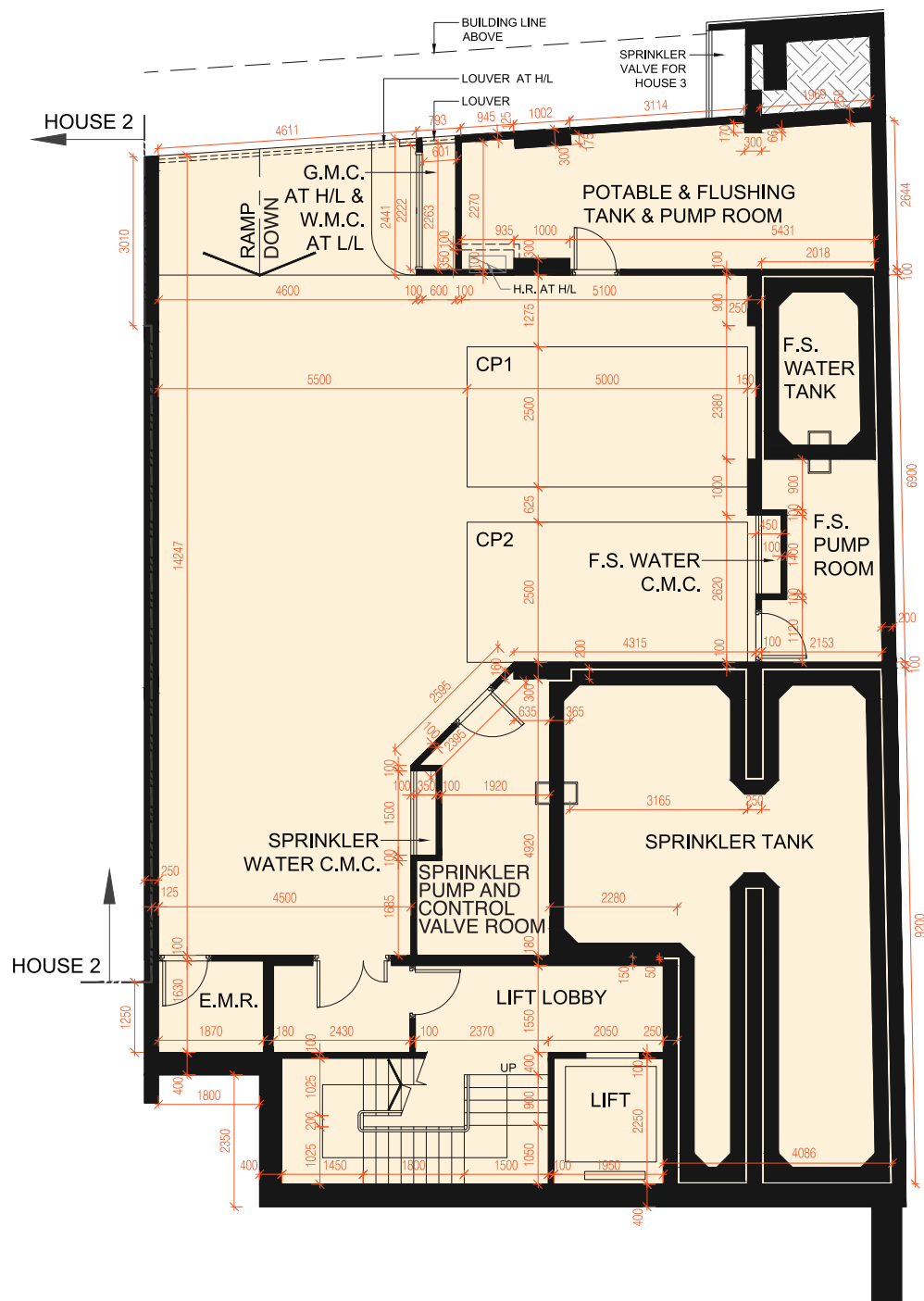
LOWER GROUND FLOOR PLAN 低層地下平面圖
