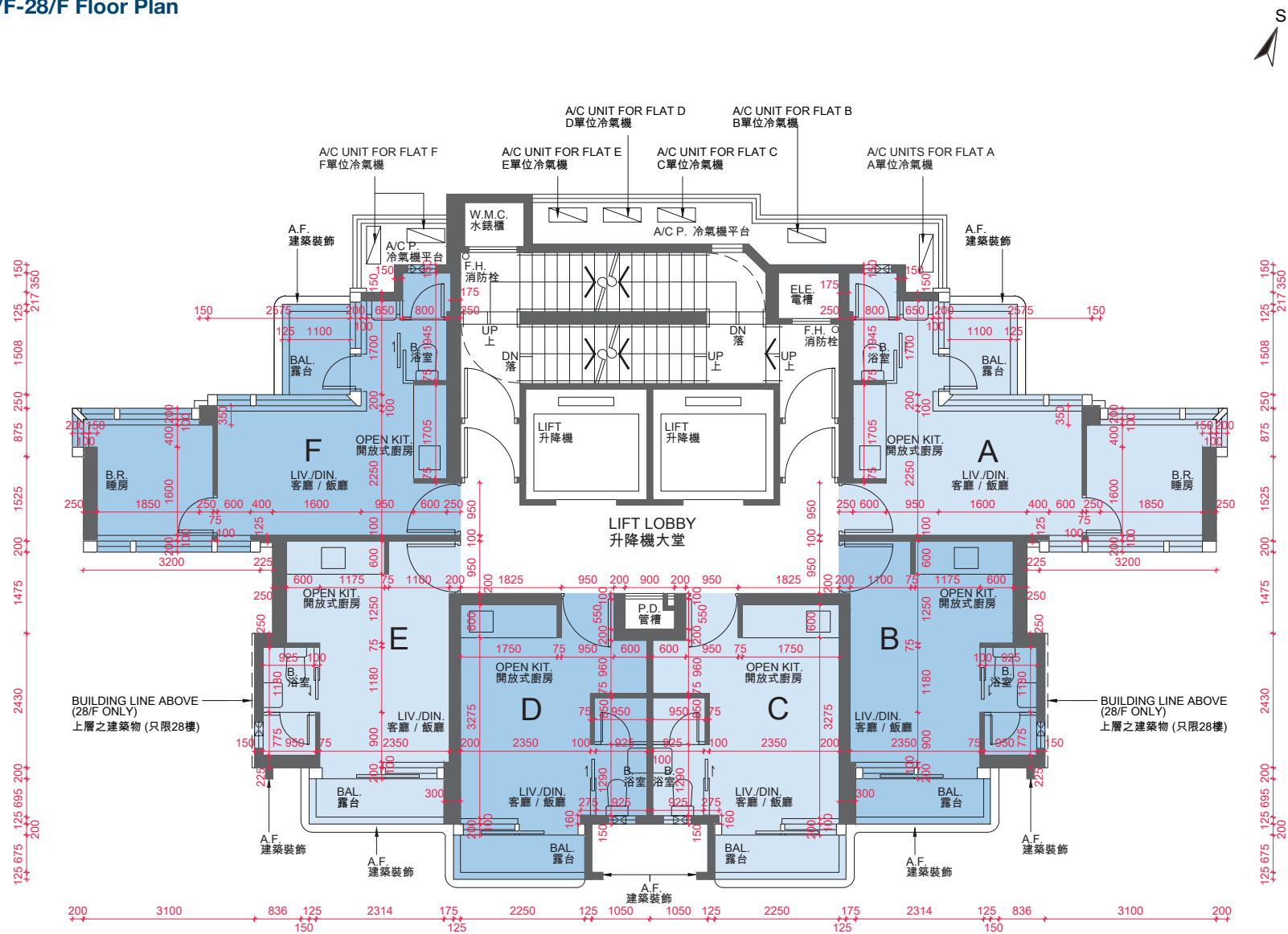
16樓-23樓、25樓-28樓平面圖 16/F-23/F, 25/F-28/F Floor Plan
