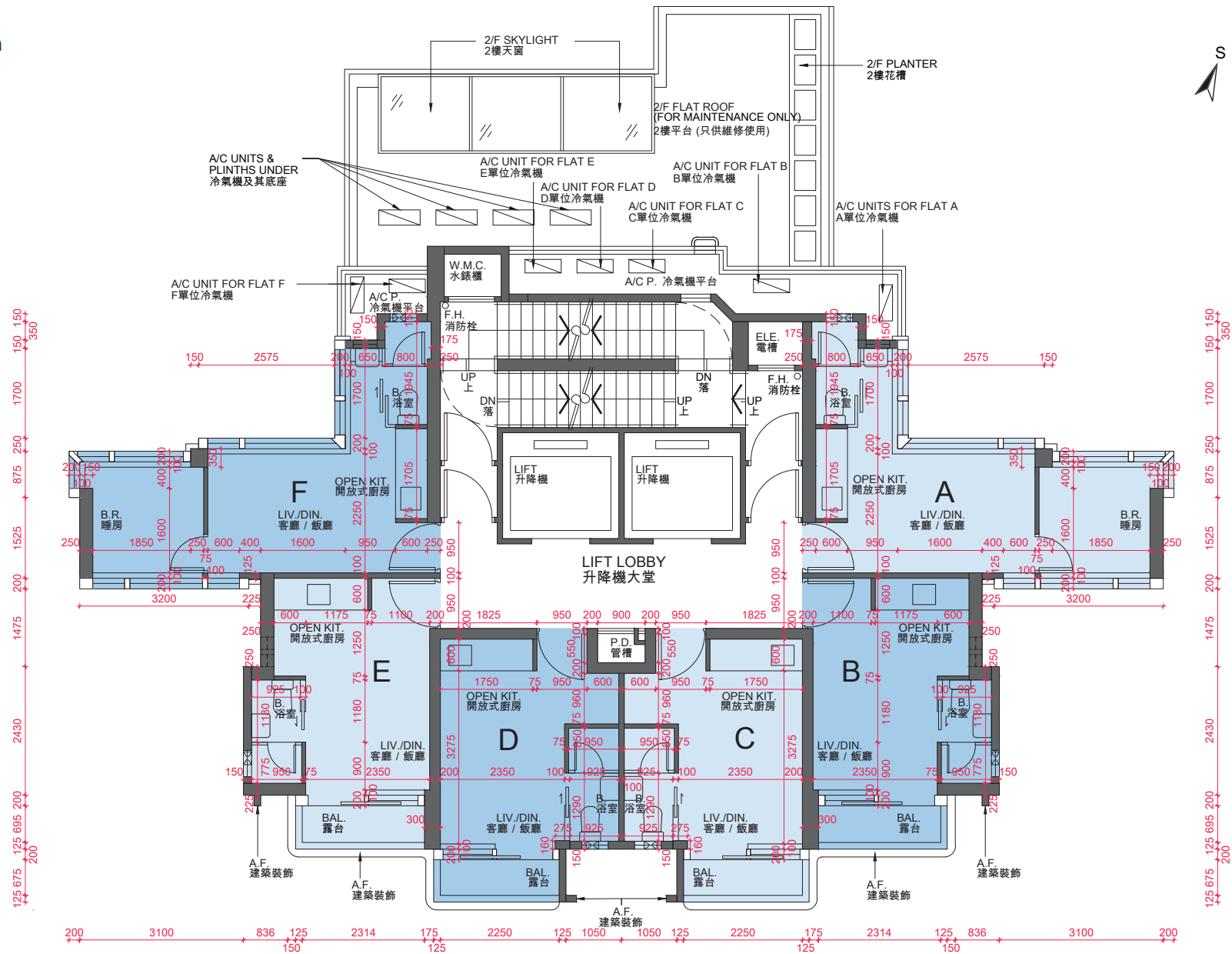
3樓平面圖 3/F Floor Plan
