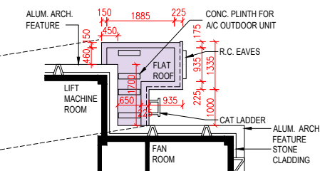
Plant Room Floor Part Plan 機電層局部平面圖
