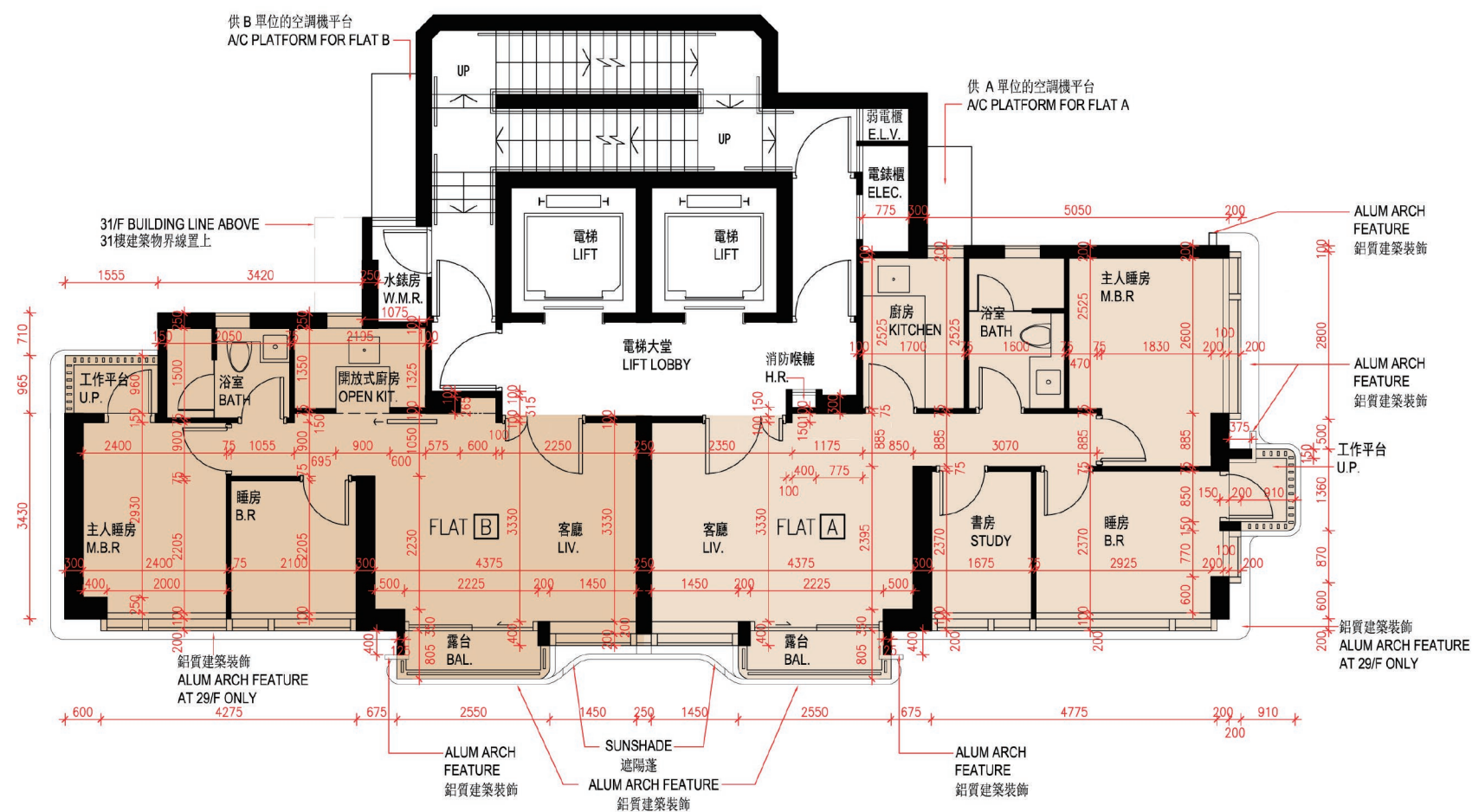
PART PLAN OF 29/F 29樓部分平面圖
