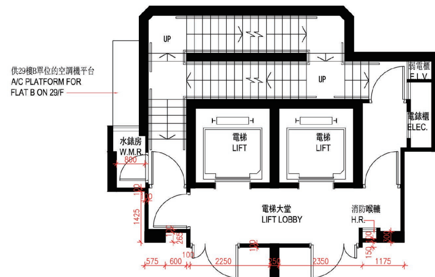
PART PLAN OF 29/F 29樓部分平面圖
