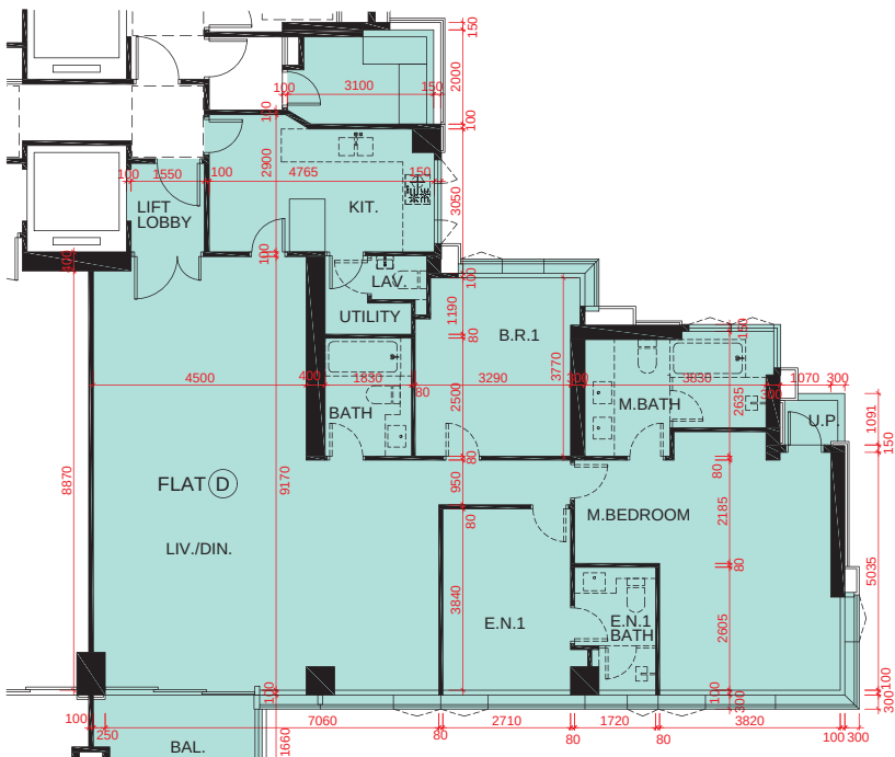
9/F FLAT D FLOOR PLAN 9樓單位D平面圖
